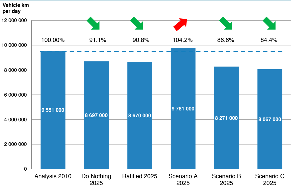
Figure 18: Projected traffic volume for different VEP scenarios in the city of Dresden (car-km per day). Source: Landeshauptstadt Dresden, 2013
