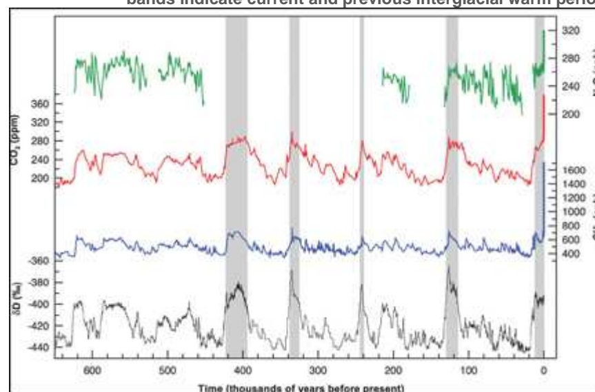
Figure 2.3: Variations of deuterium (δD) in Antarctic ice, and of carbon dioxide (CO 2 ), methane (CH 4 ) and nitrous oxide (N 2 O) in air trapped within ice cores. Shaded bands indicate current and previous interglacial warm periods.
