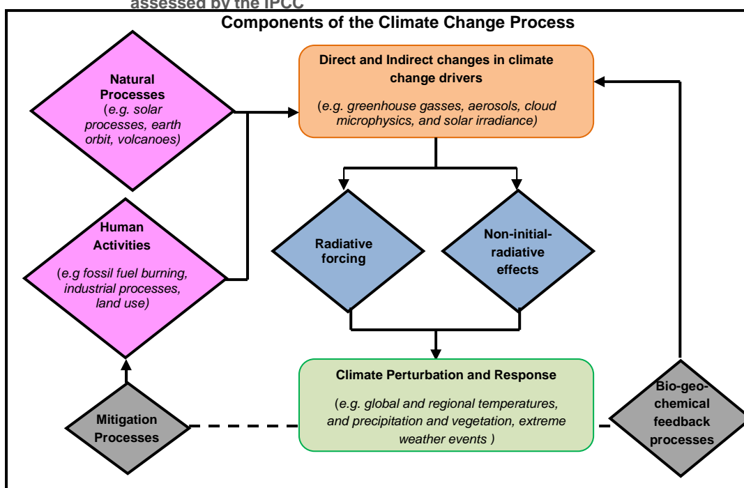
Figure 2.6: Diagram illustrating how RF is linked to other aspects of climate change assessed by the IPCC
